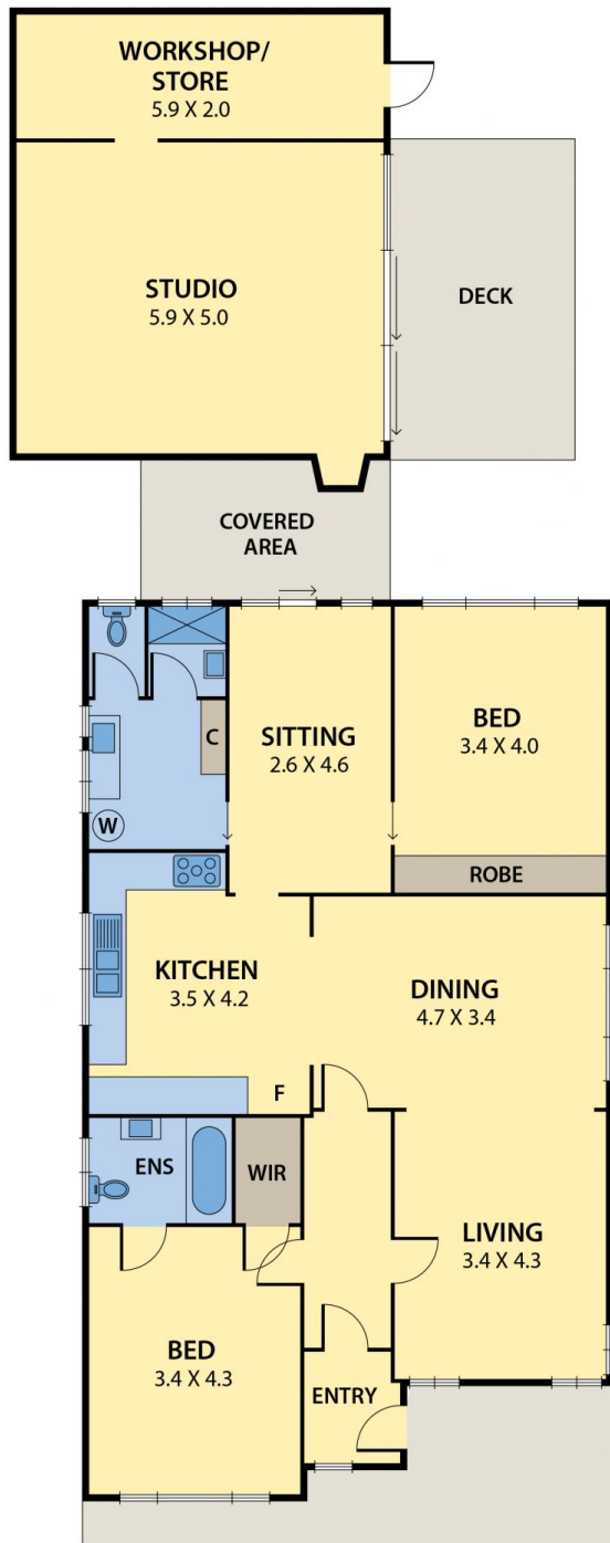
FLOOR PLAN
