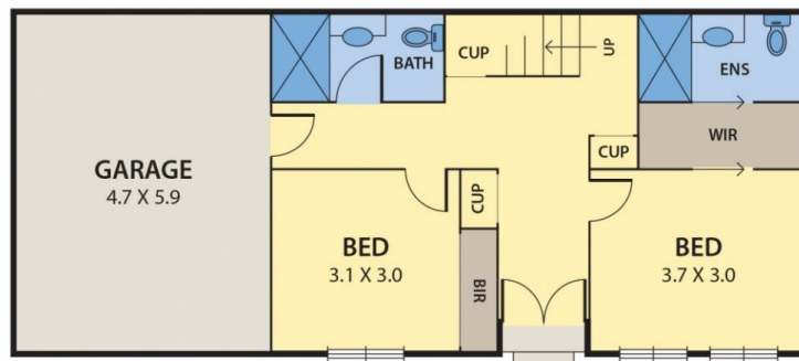
GROUND FLOOR
